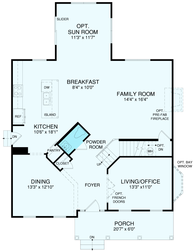
FIRST FLOOR PLAN W/ SUNROOM
