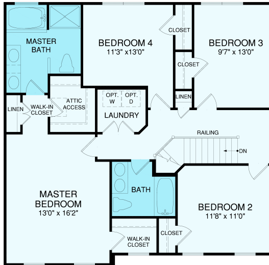
SECOND FLOOR 4 BEDROOM PLAN
